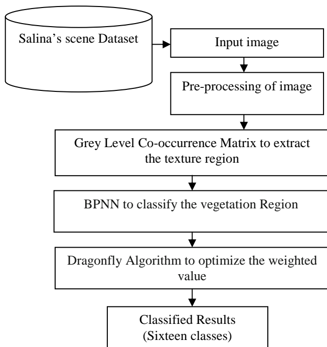
Figure 1 F Low chart for Proposed BPNN
